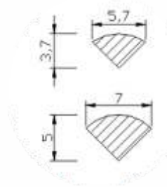
Profile welding rod continuous made of PVC-U (grey, red), PVC-P (transparent), HD-PE (black, white, natural), PE-LD (black), PP (beige, natural, white, black, blue), ABS (white, black), PP/EPDM (black), PA6, PC, Xenoy, PS, PET-G
